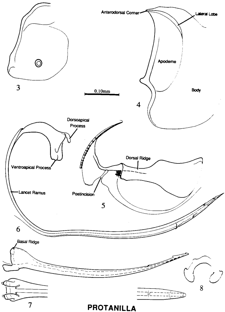
Figures 3-8. Sting apparatus of Protanilla sp. worker. 3. Lateral spiracular plate: dorsal view medial connection (part). 4. Lateral quadrate plate. 5. Lateral oblique plate, with dorsal view of dorsal ridge. Lower parts of ramus and ventral arm missing. 6. Lateral triangular plate and lancet. 7. Above: lateral sting. Below: ventral views of proximal and distal ends of sting. 8. Anterior view of furcula. All figures to same scale.
