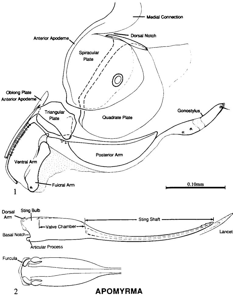
Figures 1-2. Sting apparatus of Apomyrma stygia workers. 1. Lateral views of spiracular, quadrate, oblong plates and gonostylus. Spiracular and quadrate plates have been moved dorsad to reveal underlying plates. 2. Above: lateral sting, furcula and end of lancet. Below: ventral furcula and anterior half of sting. All figures to same scale.
